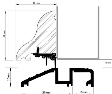
TJ Threshold with WC weatherboard
