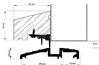
TH Threshold with WB weatherboard
