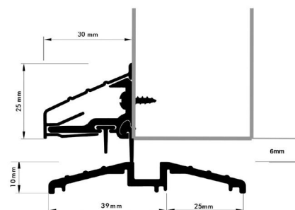
TK threshold with WA weatherboard
