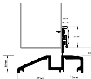
TJ threshold with CA contact strip
