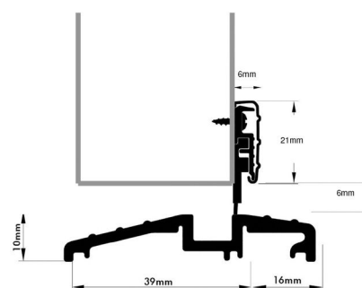
TH threshold with CA contact strip
